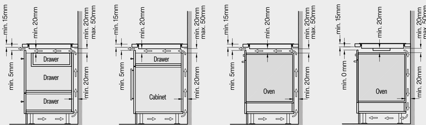
Minimum distances for the correct ventilation
